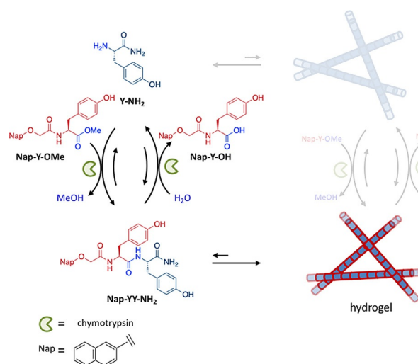
Figure 10. Transient self-assembly of a hydrogel caused by the enzyme-mediated activation and deactivation of C-terminal-amidated L-tyrosine ( \text{Y-NH}_2 ).
