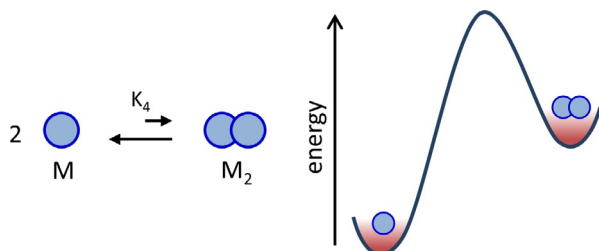
Figure 1. The equilibrium between M and M_2 that is used as a reference throughout the Review. The composition at equilibrium is defined by the equilibrium constant K_4 ( M^{-1} ). The notation for the equilibrium constant ( K_4 ) is used to facilitate the comparison of the discussion in this Review with a previous publication. [62]
